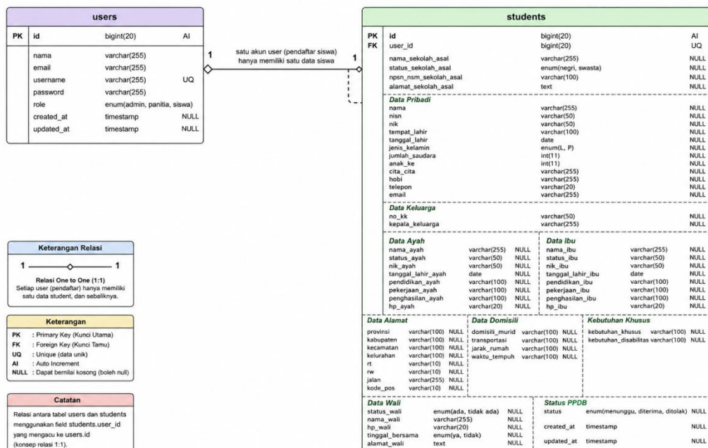
Gambar 3.9 class diagram
